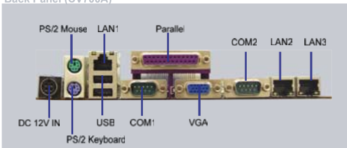
Back Panel (CV700A)
